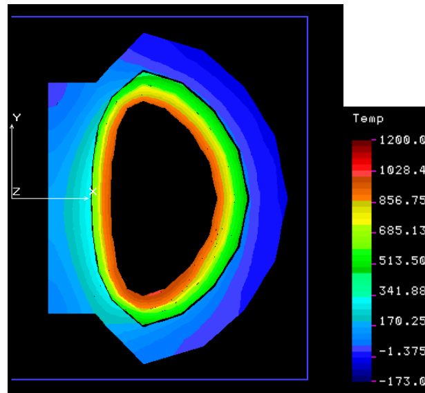
Fig. 10: Temperature profile in a poloidal cross-section of PPCS Model A, 10 days after the onset of a hypothetical bounding accident in which a total loss of all coolant is postulated, together with the failure of all active safety systems. The temperatures are in degree Celsius and Y denotes the vertical direction.
